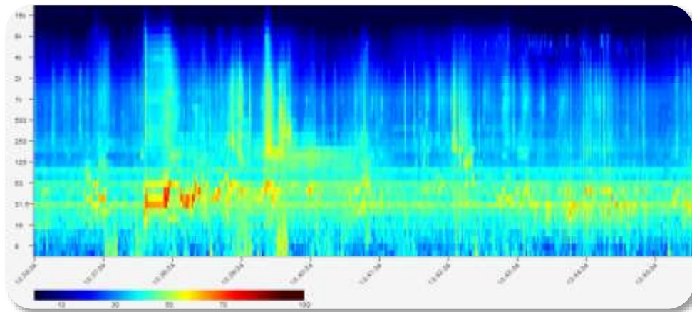
Figure 12: Real-time Spectrogram
